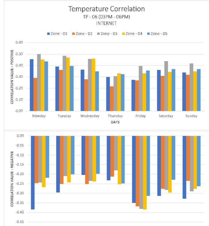
Fig. 11. Day wise average +VE and -VE correlation values of zones over week at time slot 03AM – 06PM
