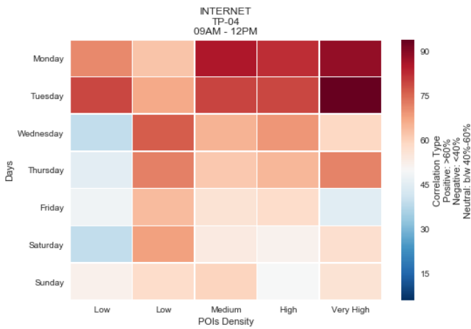
Fig. 9. Zones Heat map: Change in correlation pattern over the week at time slot 09AM – 12PM
